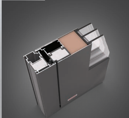
5 CarbonCore profile
